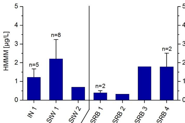
Figure 5: (Mean) concentrations and standard deviations of HMMM in the influent of StW1 (IN), stagnant waters (StW), and storm water retention basins (SRB)
